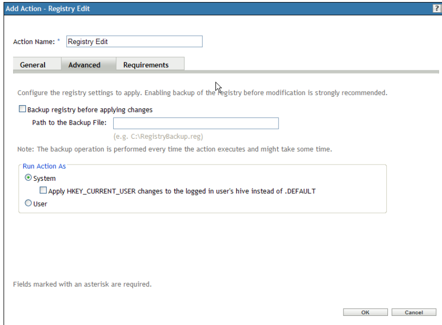
Figure 6-30 Action - Registry Edit Dialog Box: Advanced Settings Page
